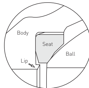
ANTI CREEP FLOW FEATURE
