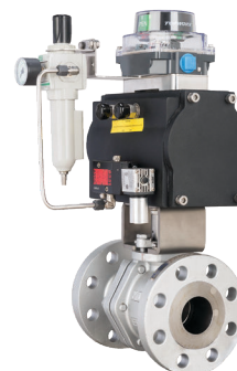
SERIES EB1 WITH F89U ACTUATOR
